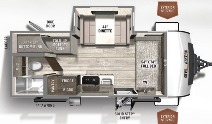
20BHS BUNKHOUSE UVW: 3513 HITCH: 455 AXLE: 3020 CCC: 842 LENGTH: 21' 2" WIDTH: 7' 8" GEO PRO HEIGHT: 10' INT. HEIGHT: 6' 6" FRESH: 31 gal GRAY: 30 gal BLACK: 30 gal
