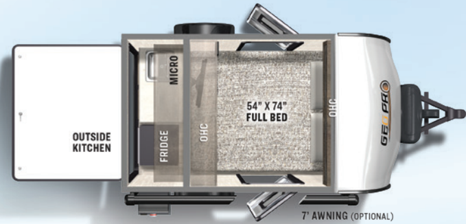
12RK REAR KITCHEN U/VW: 1252 HITCH: 162 AXLE: 1052 CCC: 710 LENGTH: 11'3" WIDTH: 6'8" GEO PRO HEIGHT: 7'9" INT. HEIGHT: 4'10" FRESH: 20 gal GRAY: 6 gal BLACK: NA
