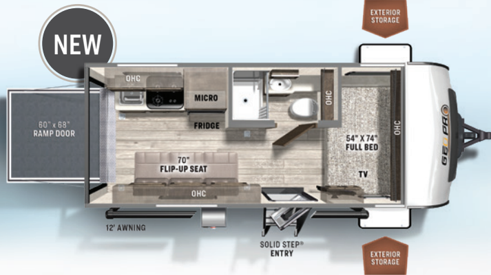
19FBTH TOY HAULER UVW: 3873 HITCH: 620 AXLE: 3215 CCC: 1097 LENGTH: 20' 2" WIDTH: 7' 8" GEO PRO HEIGHT: 10' INT. HEIGHT: 6' 6" FRESH: 31 gal GRAY: 16 gal BLACK: 30 gal
