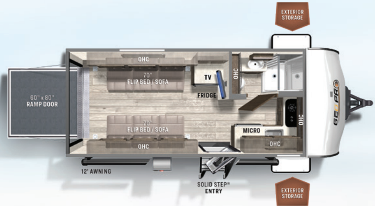
19TH TOY HAULER UVW: 3407 HITCH: 641 AXLE: 2728 CCC: 1584 LENGTH: 20' 2" WIDTH: 7' 8" GEO PRO HEIGHT: 10' INT. HEIGHT: 6' 6" FRESH: 31 gal GRAY: 16 gal BLACK: 30 gal
