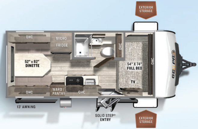
19RD REAR DINETTE UVW: 3271 HITCH: 436 AXLE: 2797 CCC: 1065 LENGTH: 20' 2" WIDTH: 7' 8" GEO PRO HEIGHT: 9' 10" INT. HEIGHT: 6' 6" FRESH: 31 gal GRAY: 30 gal BLACK: 30 gal
