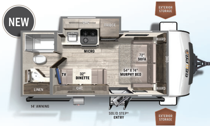
19FDS MURPHY BED UVW: 3413 HITCH: 435 AXLE: 2940 CCC: 922 LENGTH: 20' 2" WIDTH: 7' 8" GEO PRO HEIGHT: 9' 10" INT. HEIGHT: 6' 6" FRESH: 31 gal GRAY: 30 gal BLACK: 30 gal
