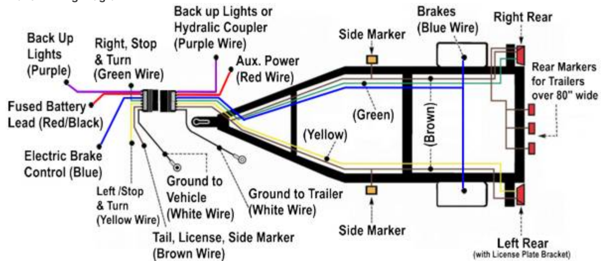
Trailer Wiring Diagram
