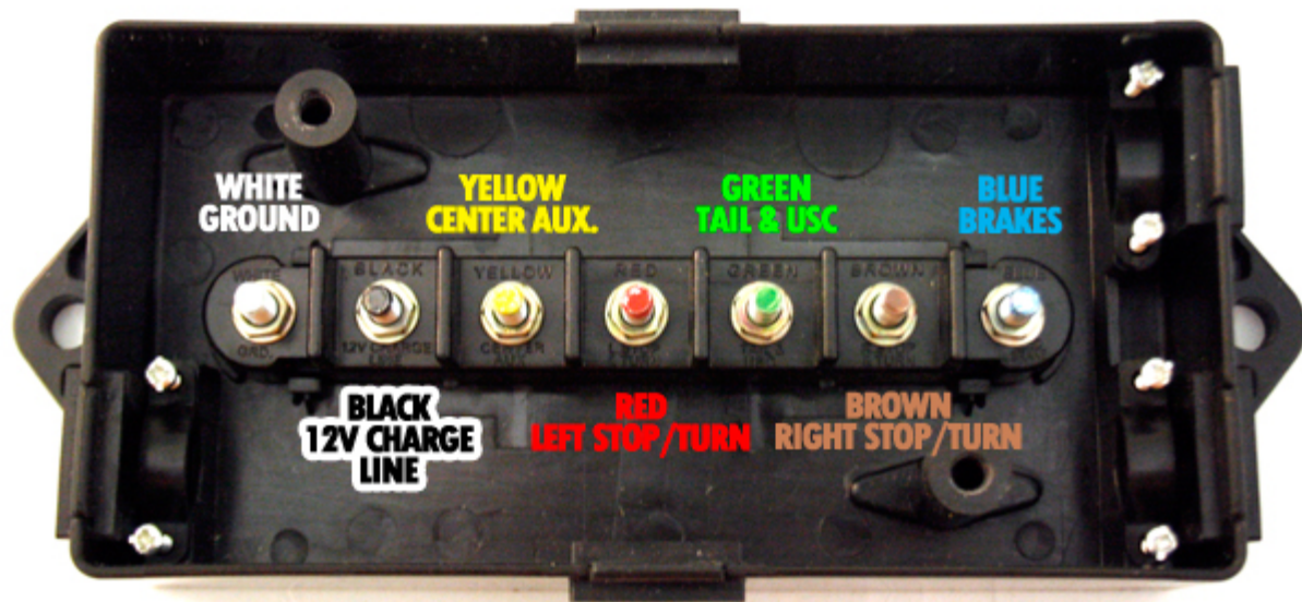
Junction Box
